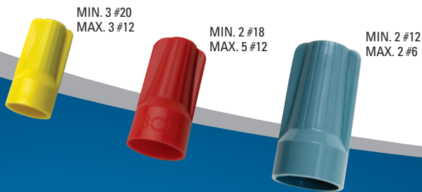
B-CAP® Wire Connector:
